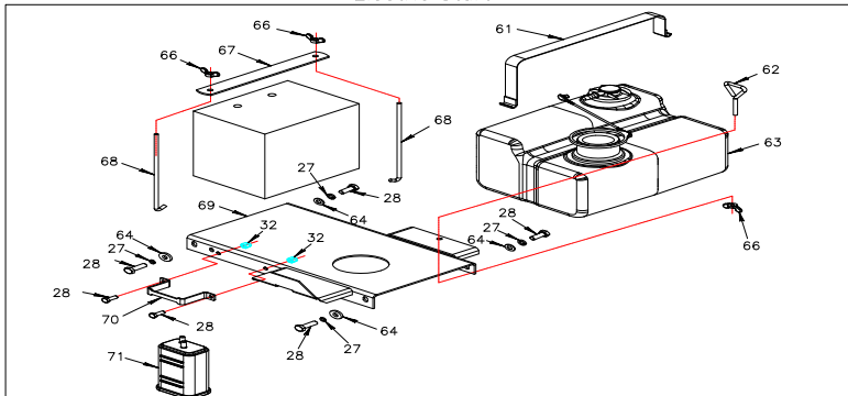
Electric Start
